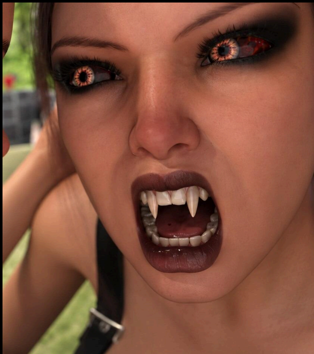
Vampire (Active)
